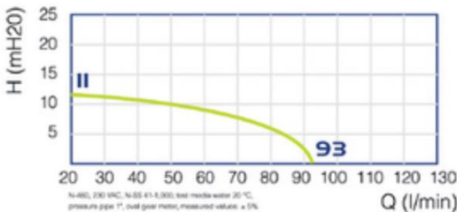
PERFORMANCE CURVE N-280
